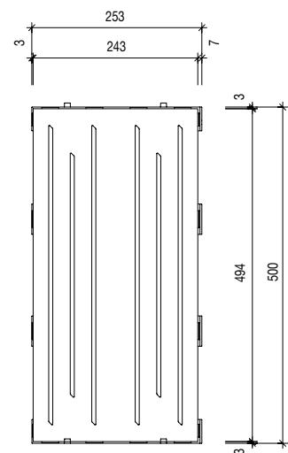
keramischer Abdeckrost ceramic cover grating
