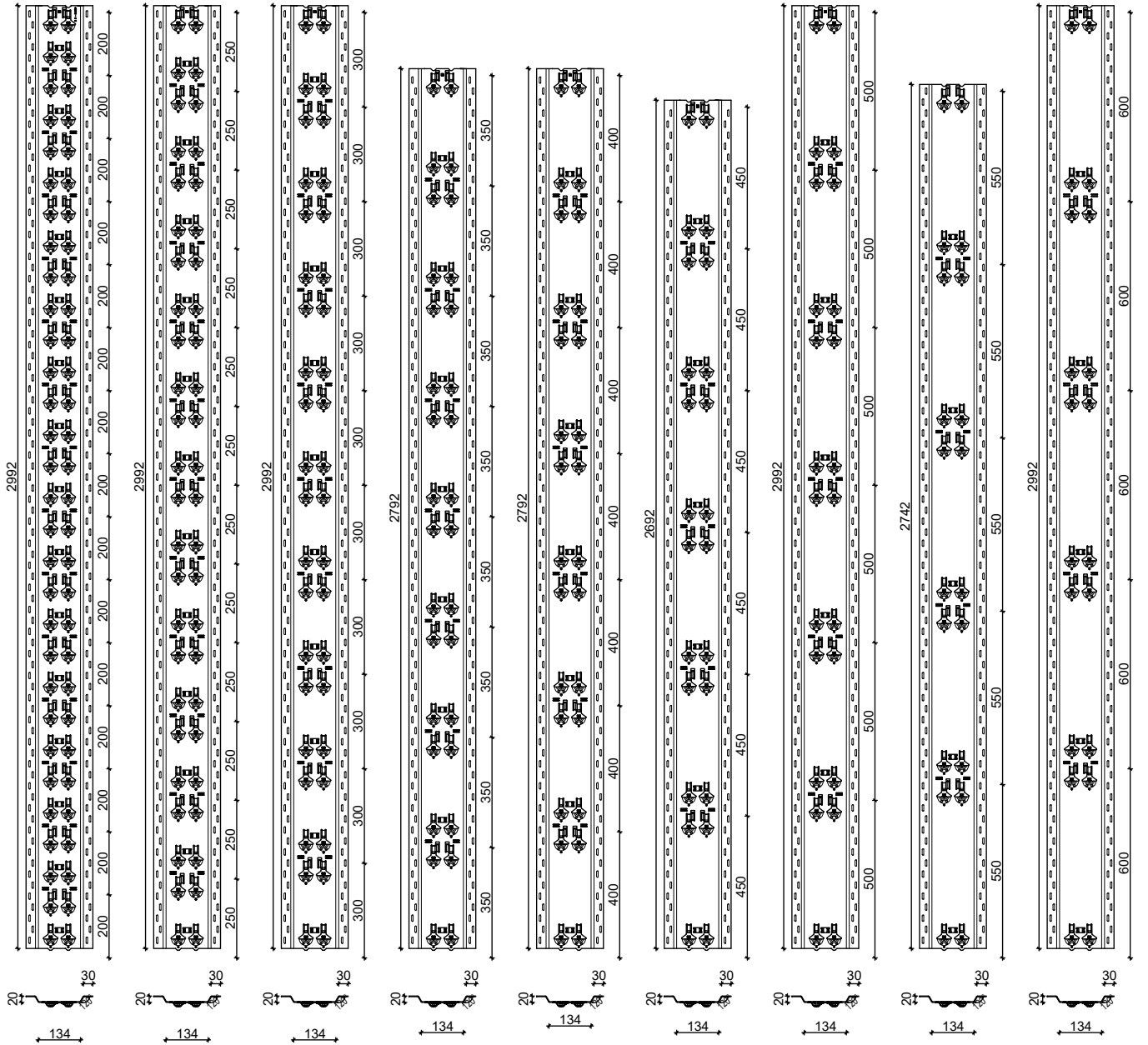
RASTER 20,0 cm 15 REIHEN RASTER 25,0 cm 12 REIHEN RASTER 30,0 cm 10 REIHEN RASTER 35,0 cm 8 REIHEN RASTER 40,0 cm 7 REIHEN RASTER 45,0 cm 6 REIHEN RASTER 50,0 cm 6 REIHEN RASTER 55,0 cm 5 REIHEN RASTER 60,0 cm 5 REIHEN
