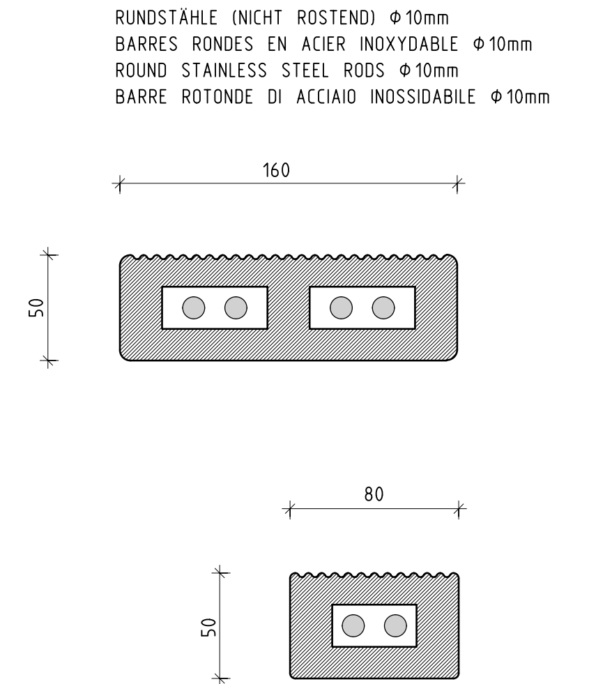
PUNKT "C" u. "D" POINT "C" + "D" / POINT "C" + "D" / PUNTO "C"+"D"
