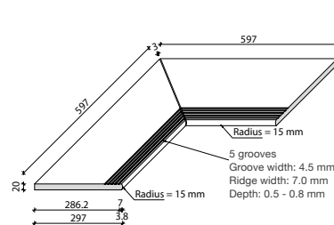
Patio tile with rounded edge on one side and grooves as corner solution (2 pieces)
