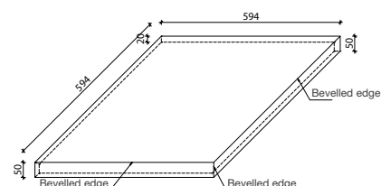
Patio tile step with nosing as corner solution
